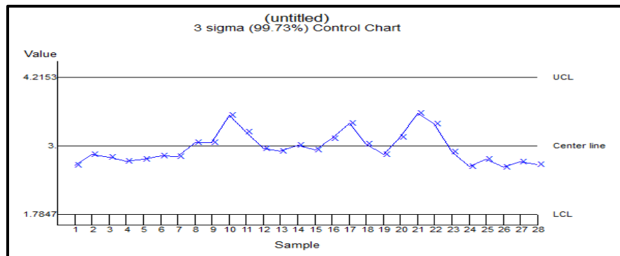
Gambar 4 Peta Kendali X ( X -Chart) Free Fatty Acid / Asam Lemak Bebas (FFA) Oil Production Line I dan II Bulan Mei 2016
