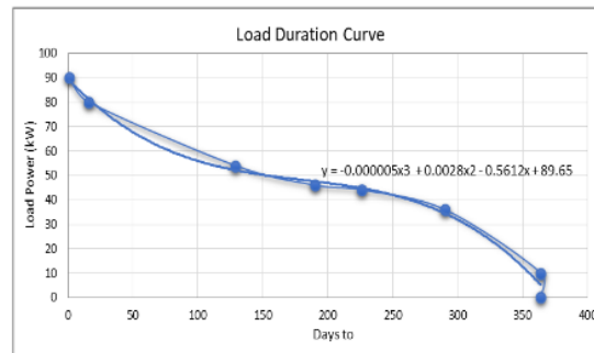
Figure 6. The electricity load duration curve with its equation served by the Pantai Baru hybrid power plant during 2018
