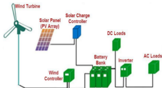
Figure 1. The typical hybrid power plants
