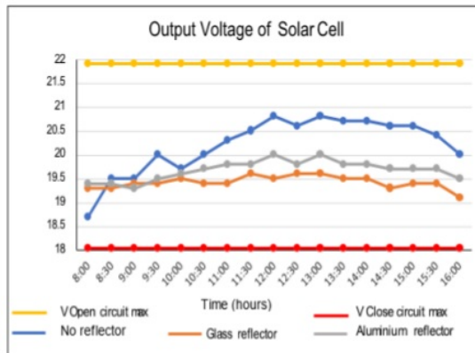
Figure 9. Output voltage of solar photovoltaic system in batik industry
