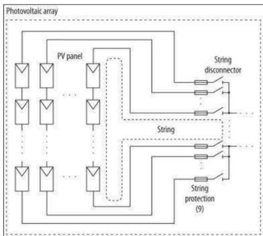
Figure 4. PV arrays arranged in parallel series
