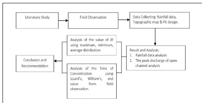
Fig. 19. Research Steps.
