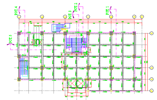
Fig. 3. floors 1-7
