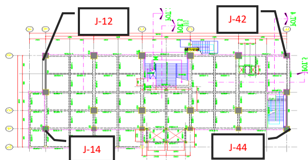
Fig. 7. Review point of displacement value
