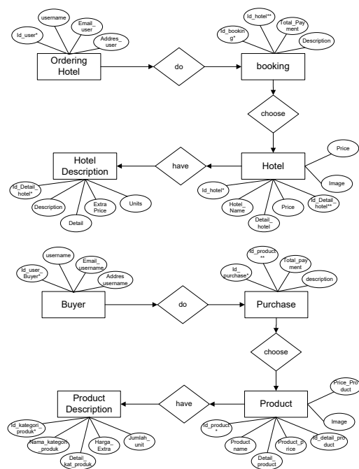
Figure 9 Database Design
