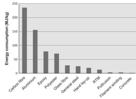
Fig. 1. Energy consumption for production of differentt materials and manufacturing process (Hammond, 2008)
