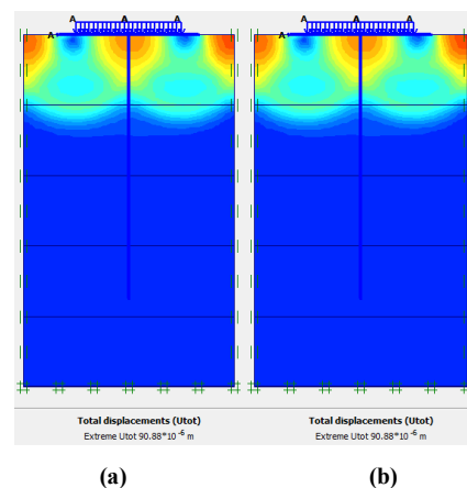
Fig. 2. (a) The results of the analysis on foundation loading phase, (b) Results of Analysis in Safety Factor phase
