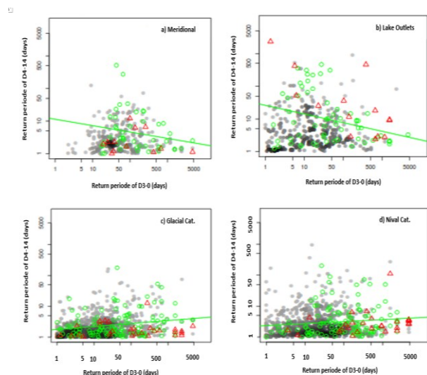
Fig. 2. Flood associated rainfall for different watershed regimes. Gray dots are annual flood. Flood return period for 5-years are indicated by green dots and Flood return period for 20-years are indicated by red triangles. Geen lines show the linear regression of the flood return period for 5-years. Source: Froidevaux et al. (2015).
