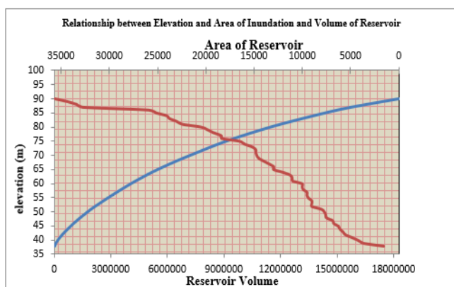
Fig. 6. Curvature of Reservoir Capacity
