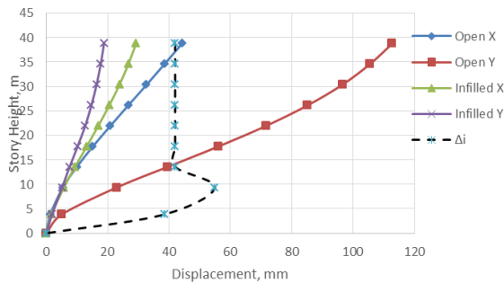
Fig. 9. Displacement curves on building joints static equivalent loads.
