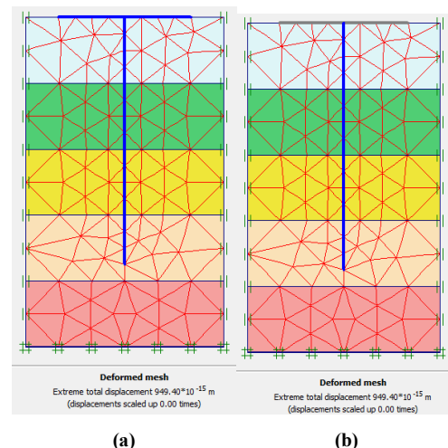
Fig. 1. (a) Results of Analysis in Foundation Installation Phase, (b) Results of Analysis in Pilecap Installation Phase
