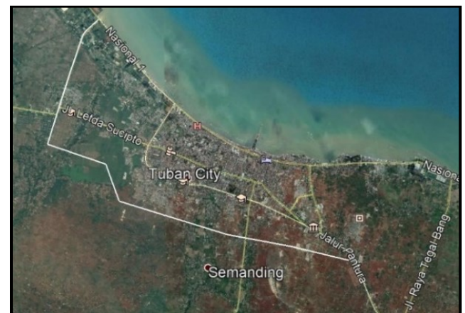
Fig. 3. Alternative 1 Ring Road Route
