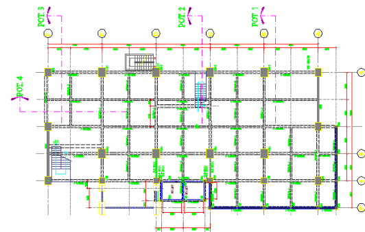
Fig. 2. Semi basement floor
