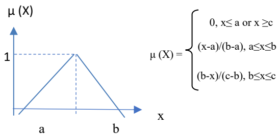
Fig. 2. Triangle Functions (Setiawan et al, 2008)
