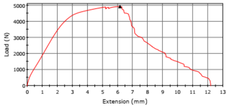
Specimen 1 to 1
