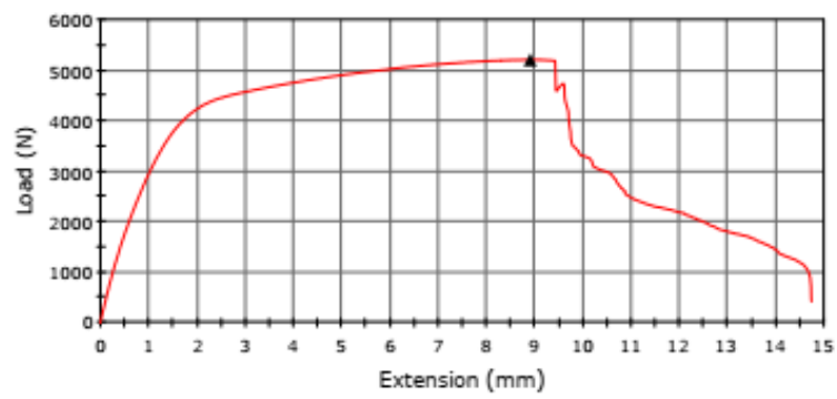
Specimen 1 to 1
