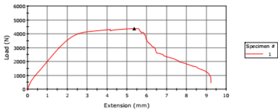
Specimen 1 to 1
