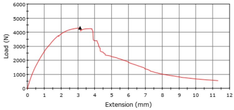
Specimen 1 to 1
