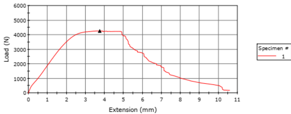
Specimen 1 to 1
