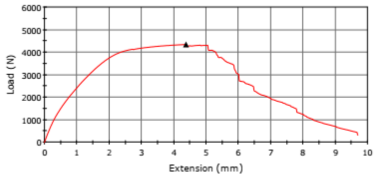
Specimen 1 to 1
