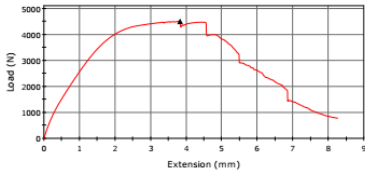
Specimen 1 to 1
