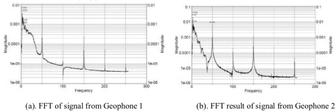
Fig. 4 – Fourier amplitude from both signals
