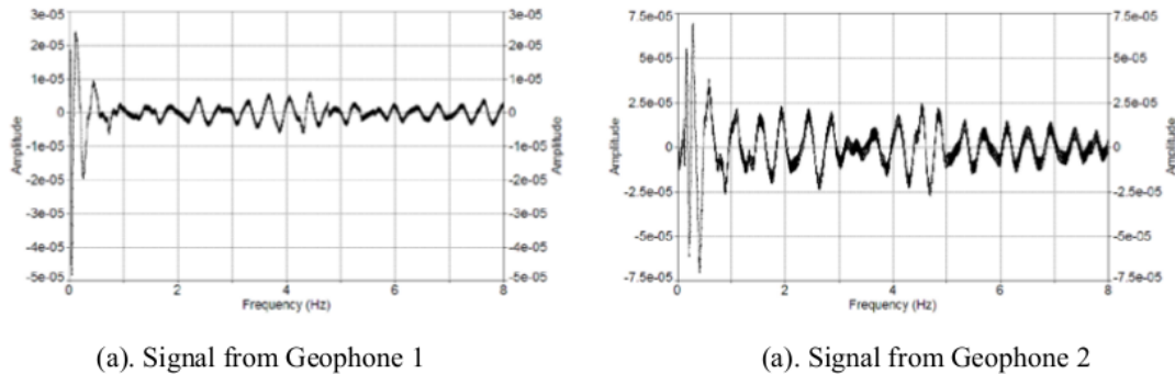
Fig. 3 – Seismic surface wave signals recorded from two channels of geophone with 8 m geophone spacing
