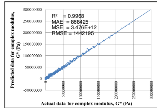
Figure 7 Graph of predicted value against actual value for complex modulus, G^* using radial basis function neural network model
