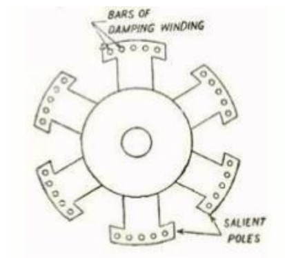
Gambar 2.5 Rotor Kutub Menonjol (Anthony, 2013)
