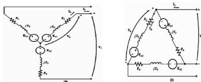
Gambar 2.10 Rangkaian Ekivalen Generator Sinkron (a) Hubung-Y (b) Hubung-D (Ramdhani, 2008)
