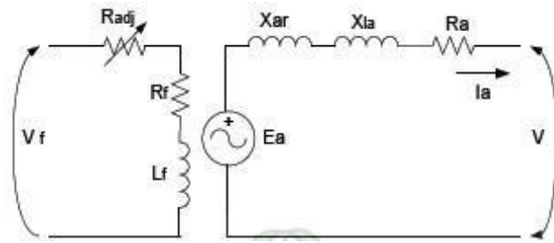
Gambar 2.7 Rangkaian Ekuivalen Generator Sinkron (Ramdhani, 2008)
