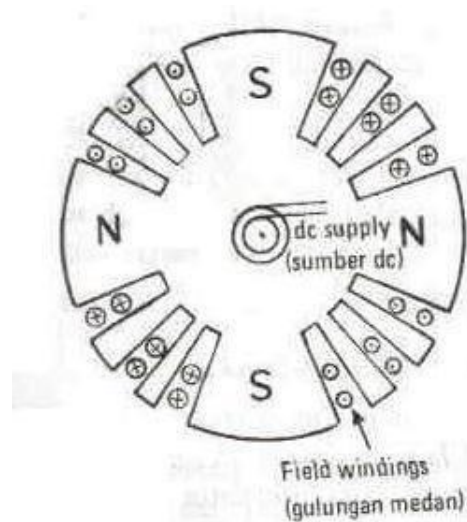
Gambar 2.6 Rotor Kutub Silinder ( Non Salient Pole )
