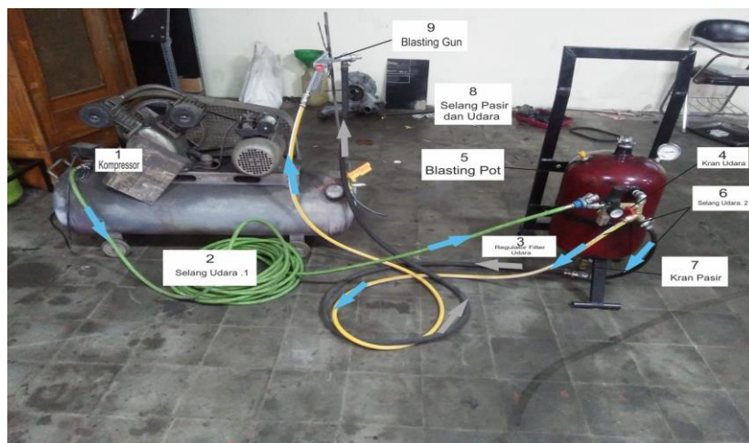
Gambar 1.2 Alat Sandblasting
