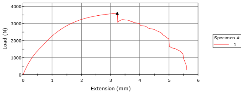
Specimen 1 to 1
