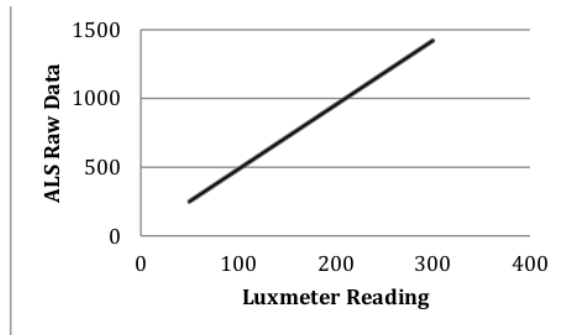
Fig. 2. Calibration Result
