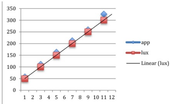
Fig. 4. Measurement Comparison
