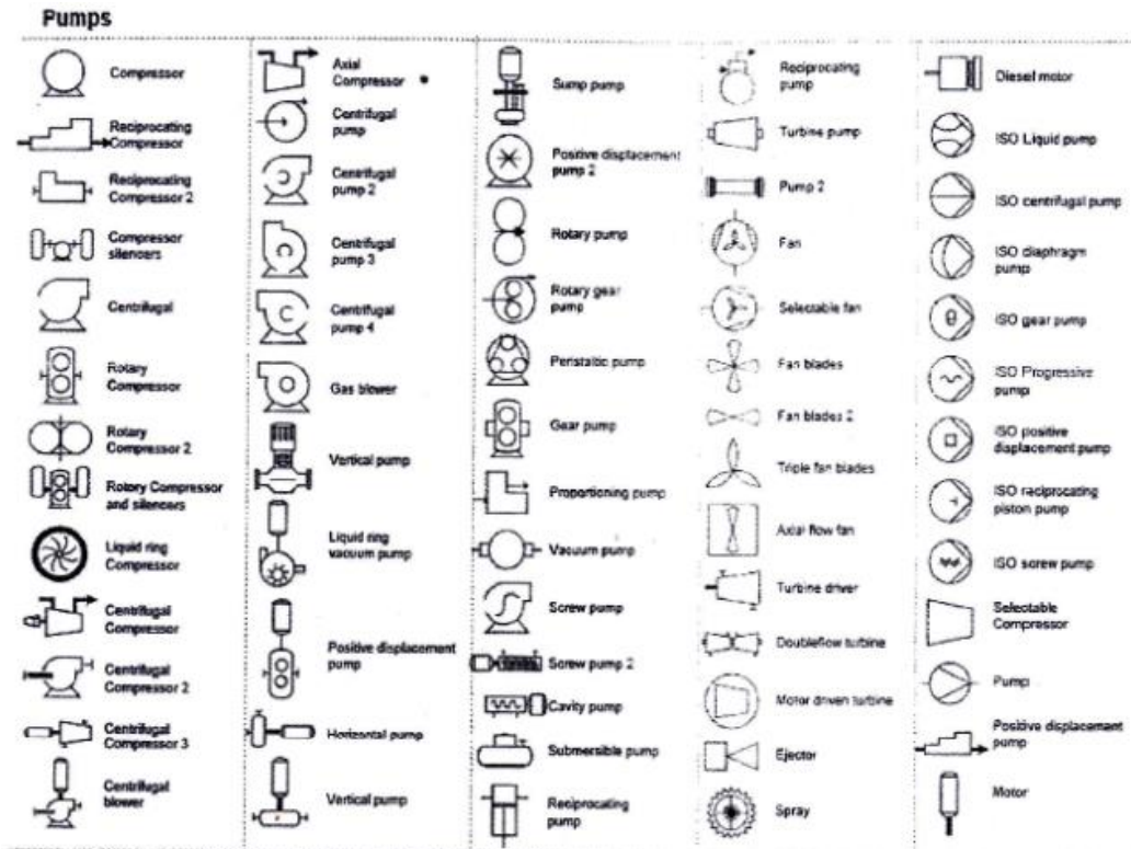
Gambar 3.26 Pump symbol
