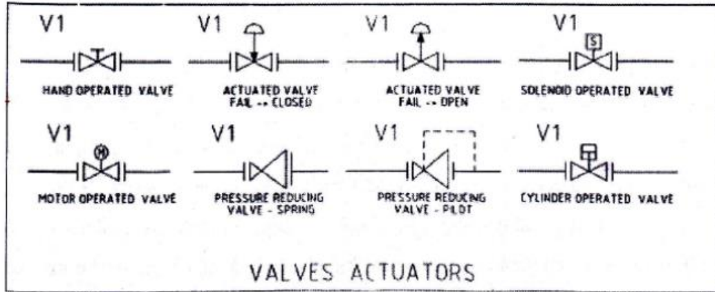
Gambar 3.24 Valve actuators symbol
