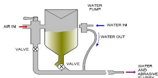
Gambar 2.3: Proses wet blasting
