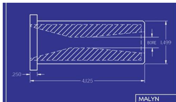
Gambar 2.5: Nozzle venturi Sumber: (Industrial supply, inc)
