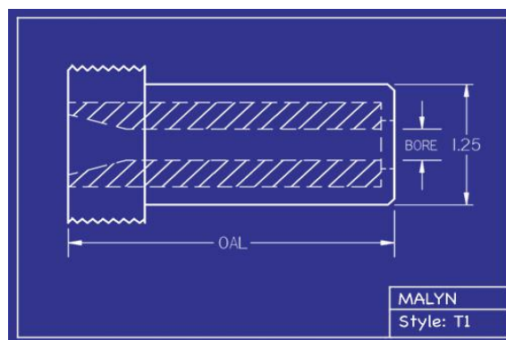
Gambar 2.4: Nozzle straight bore Sumber: (Industrial supply, inc)
