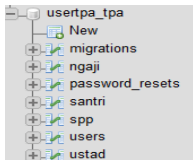
Gambar 4.1 Basis Data
