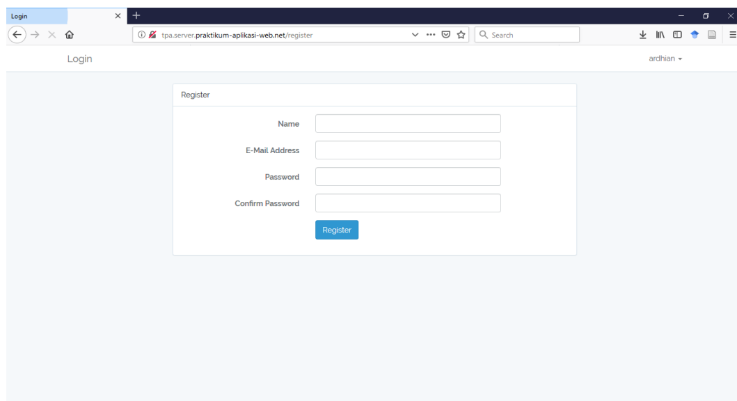
Gambar 4.28 Halaman Register
