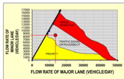
Fig. 14 - Determination of the type of intersection [10]
