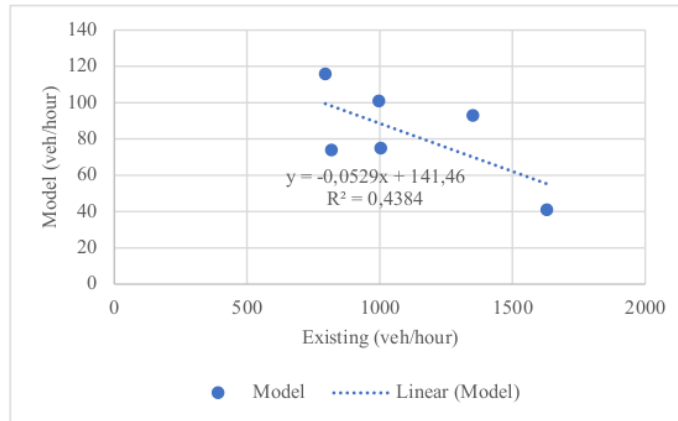
Fig. 13 – Data Validation Based On Traffic Volume
