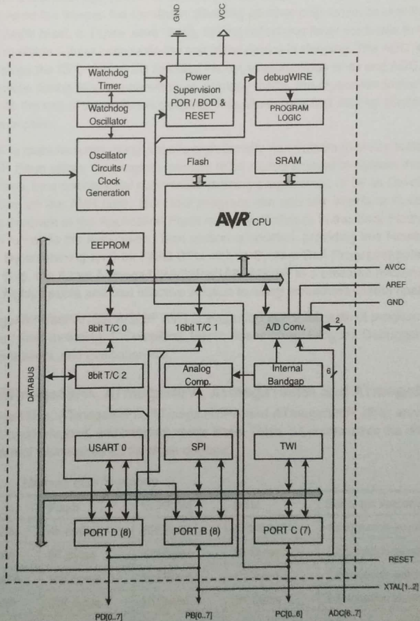
Figure 2-1. Block Diagram
