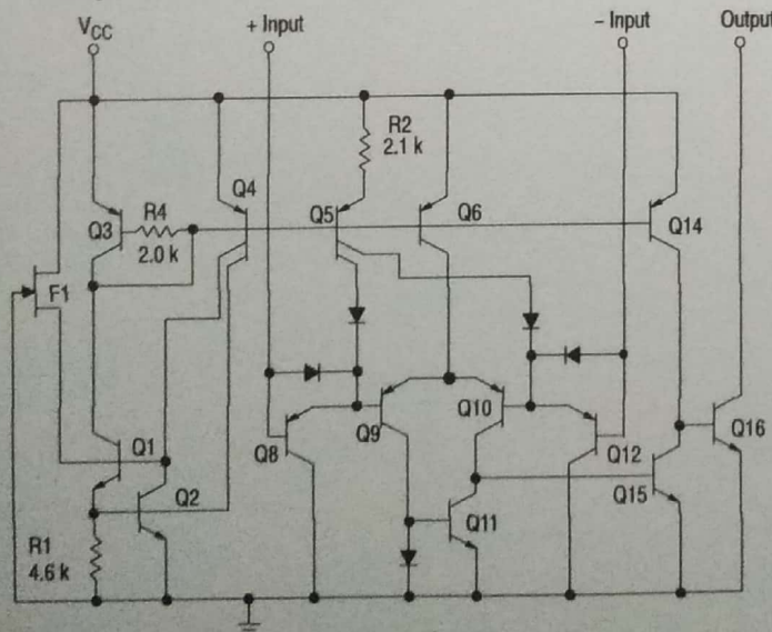
Figure 1. Representative Schematic Diagram (Diagram shown is for 1 comparator)
