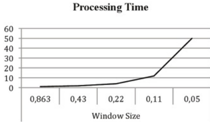
Fig. 1. Processing speed against window size
