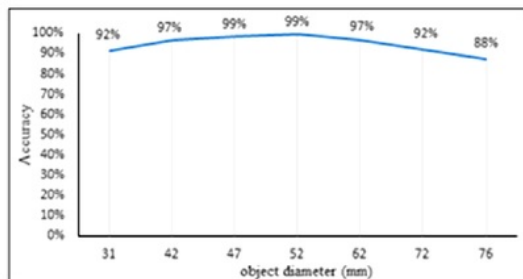
Figure 5. Accuracy of fruit measurement process using 7 spherical objects with different sizes.
