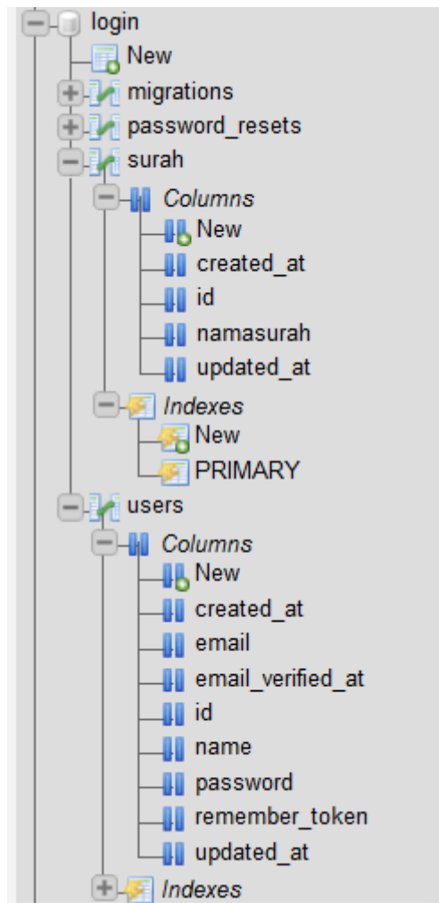
Gambar 4.1 Basis Data
