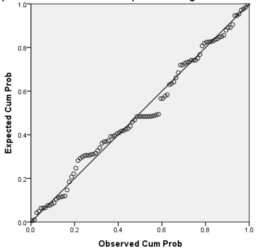
Normal P-P Plot of Regression Standardized Residual Dependent Variable: Kualitas Laporan Keuangan Pemerintah
