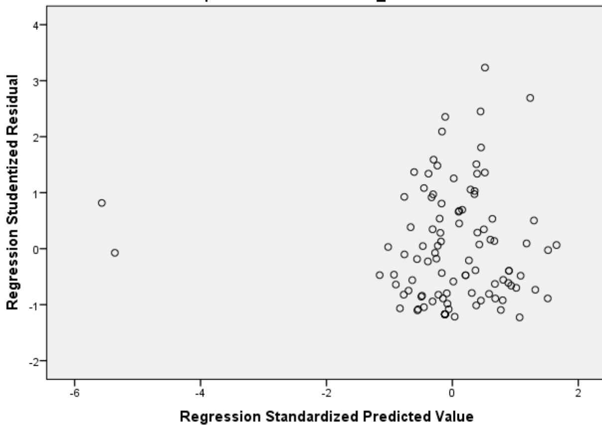
Dependent Variable: ABS_RES
