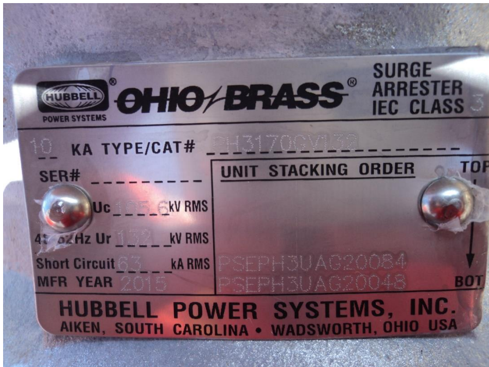
Gambar 6. Nameplate Lightning Arrester
