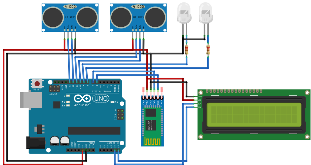
Gambar 6 Wiring Diagram System
