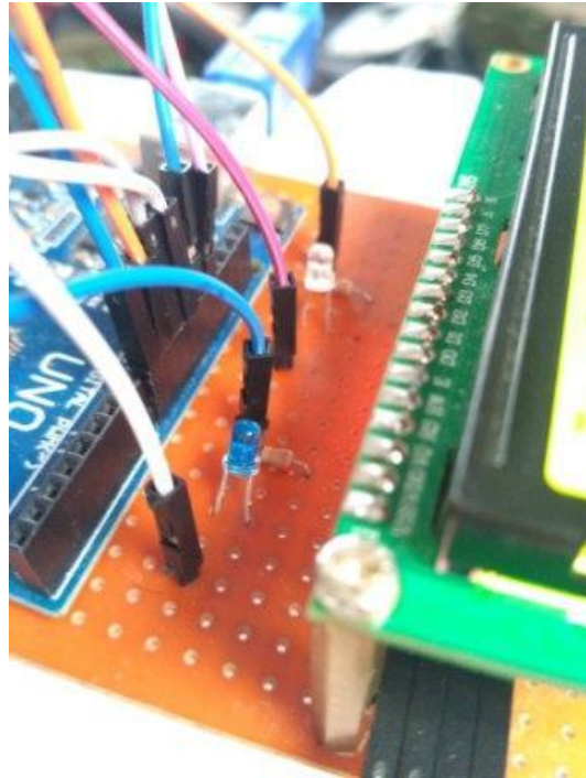
Gambar 5 Posisi LED
