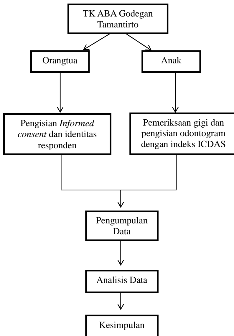
Gambar 3. Alur Penelitian
