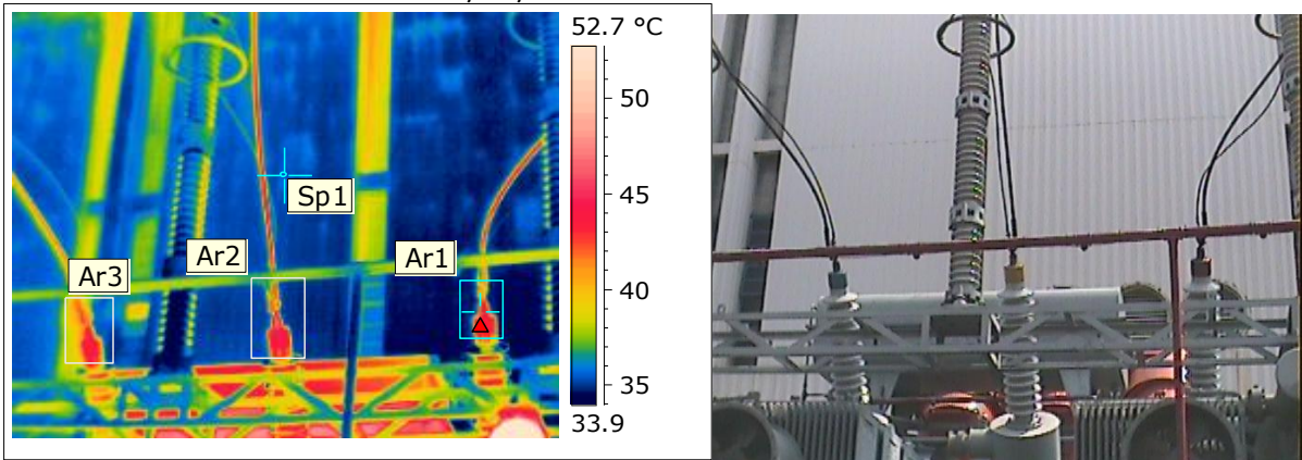
Picture 2. Captured at: Bushing
