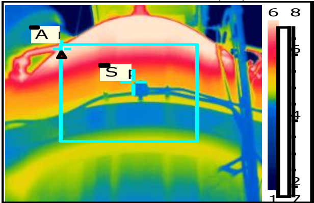
Picture 6. Captured at: dinding sisi barat
