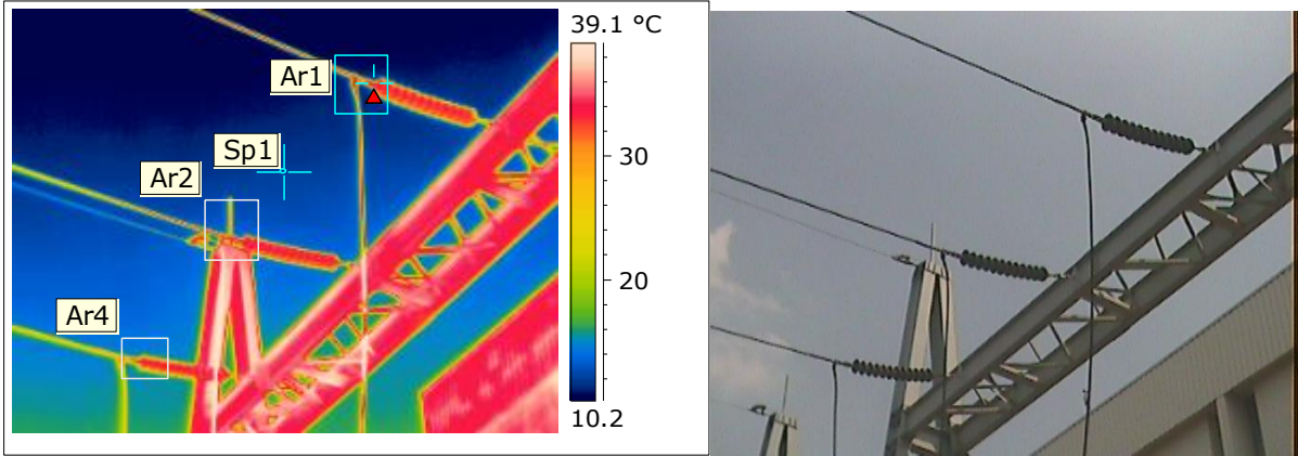
Picture 1. Captured at: Koneksi Outgoing
