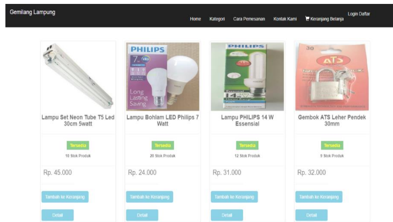
Gambar 4. 4 Halaman Home
