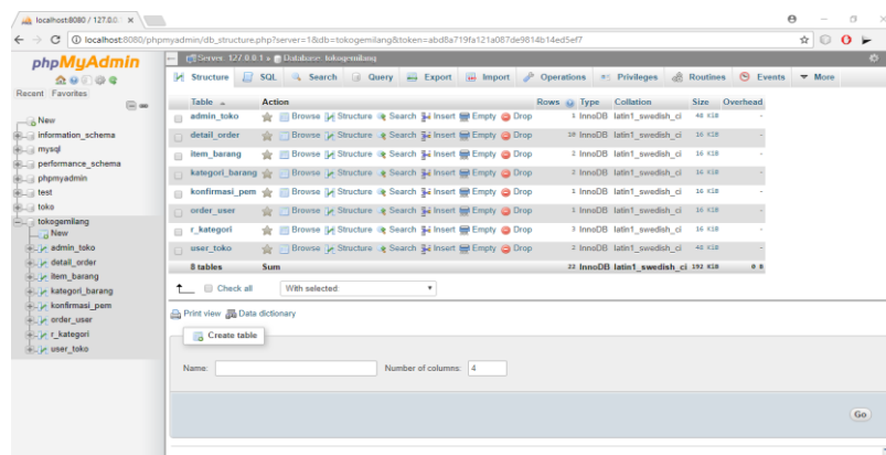
Gambar 4. 1 Database
