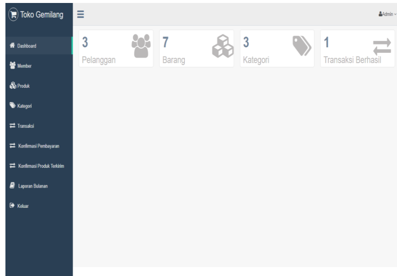
Gambar 4.15 Halaman Dashboard
