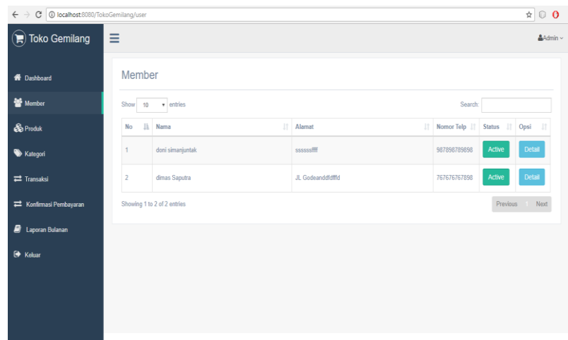
Gambar 4. 17 Halaman Member
