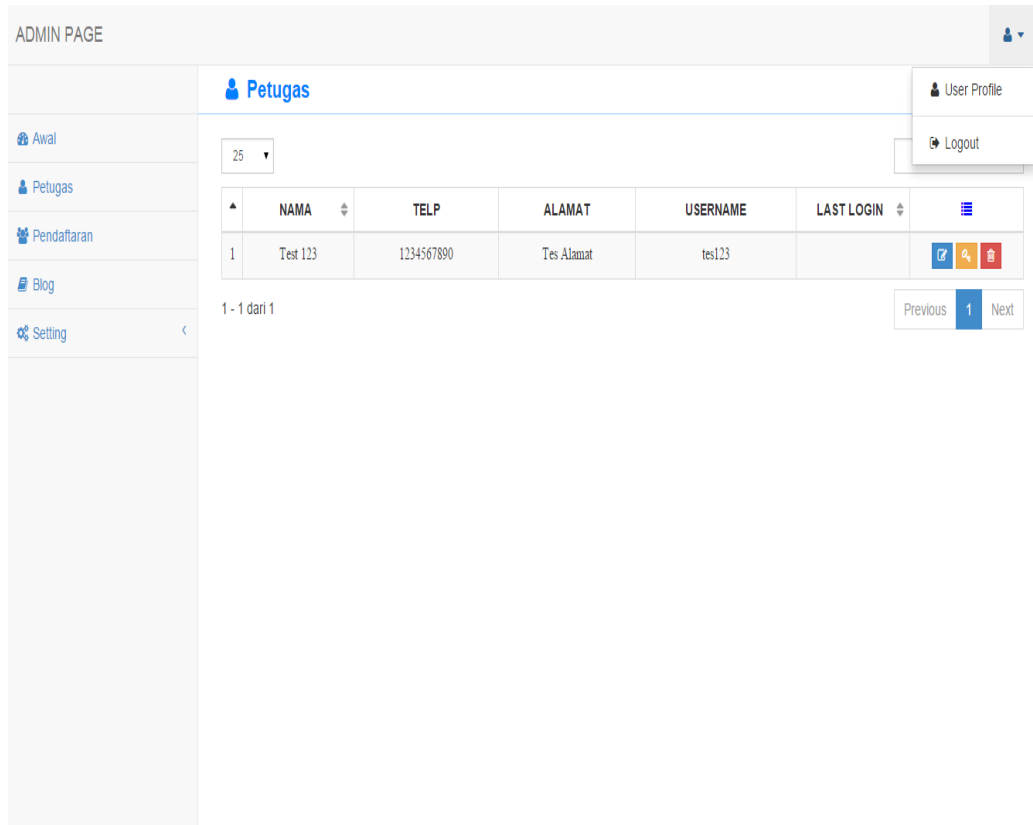
Gambar 4.13 Halaman Admin
