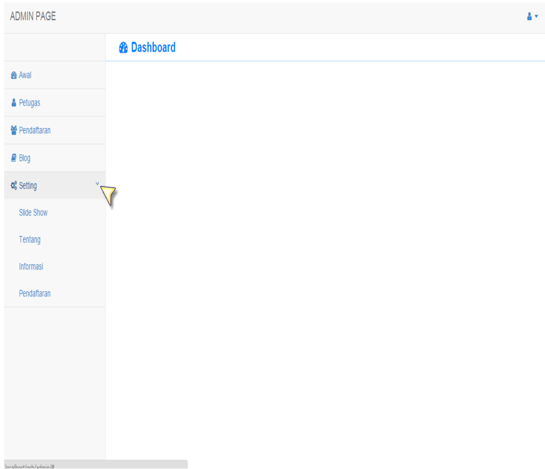
Gambar 4.16 Halaman Setting
