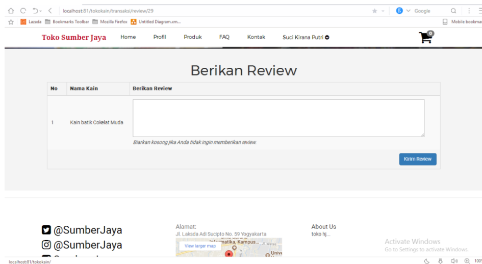
Gambar 4.20 Halaman Review
