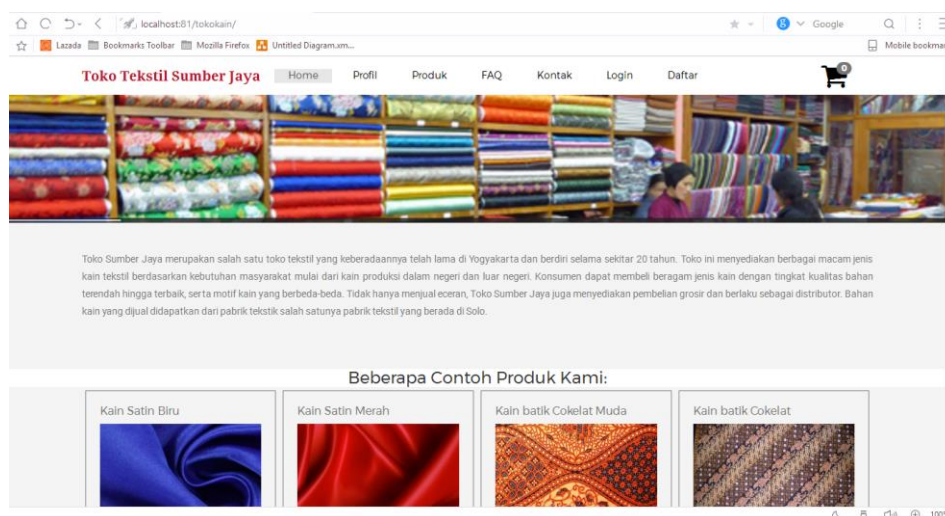
Gambar 4.11 Halaman Home
