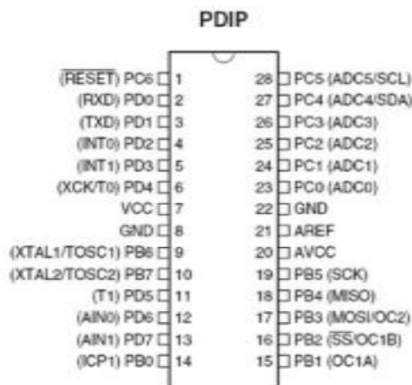
Gambar 2.3 Pin-out ATmega 8[6].
