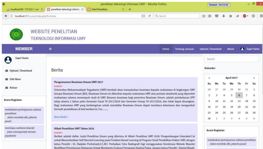
Gambar 4.10 Halaman Home
