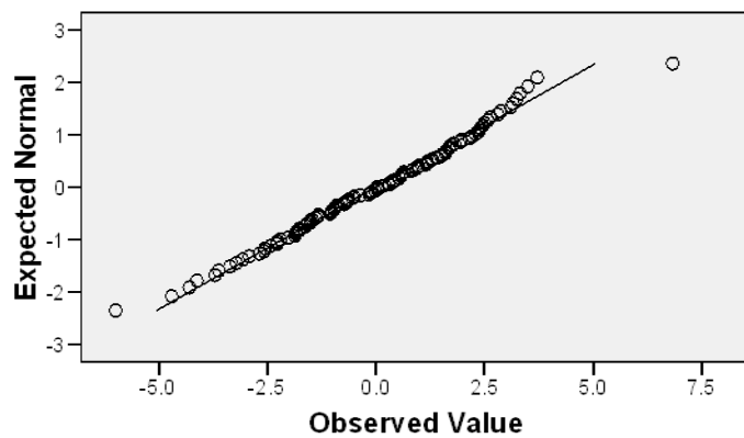
Normal Q-Q Plot of Unstandardized Residual
